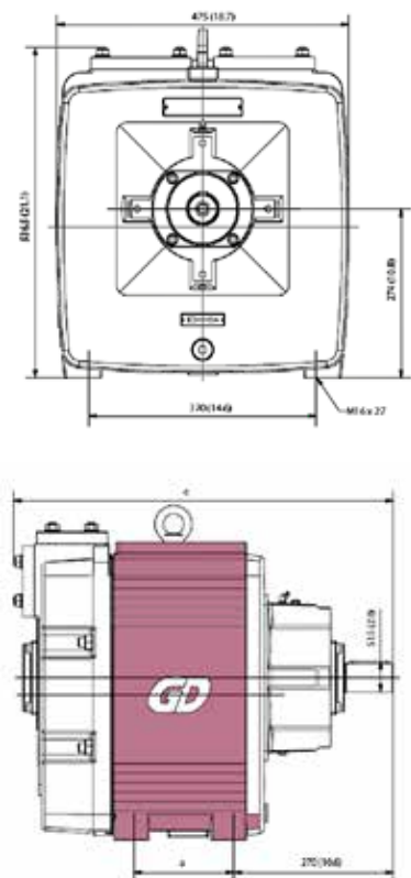
Wittig Aqualine 1200
